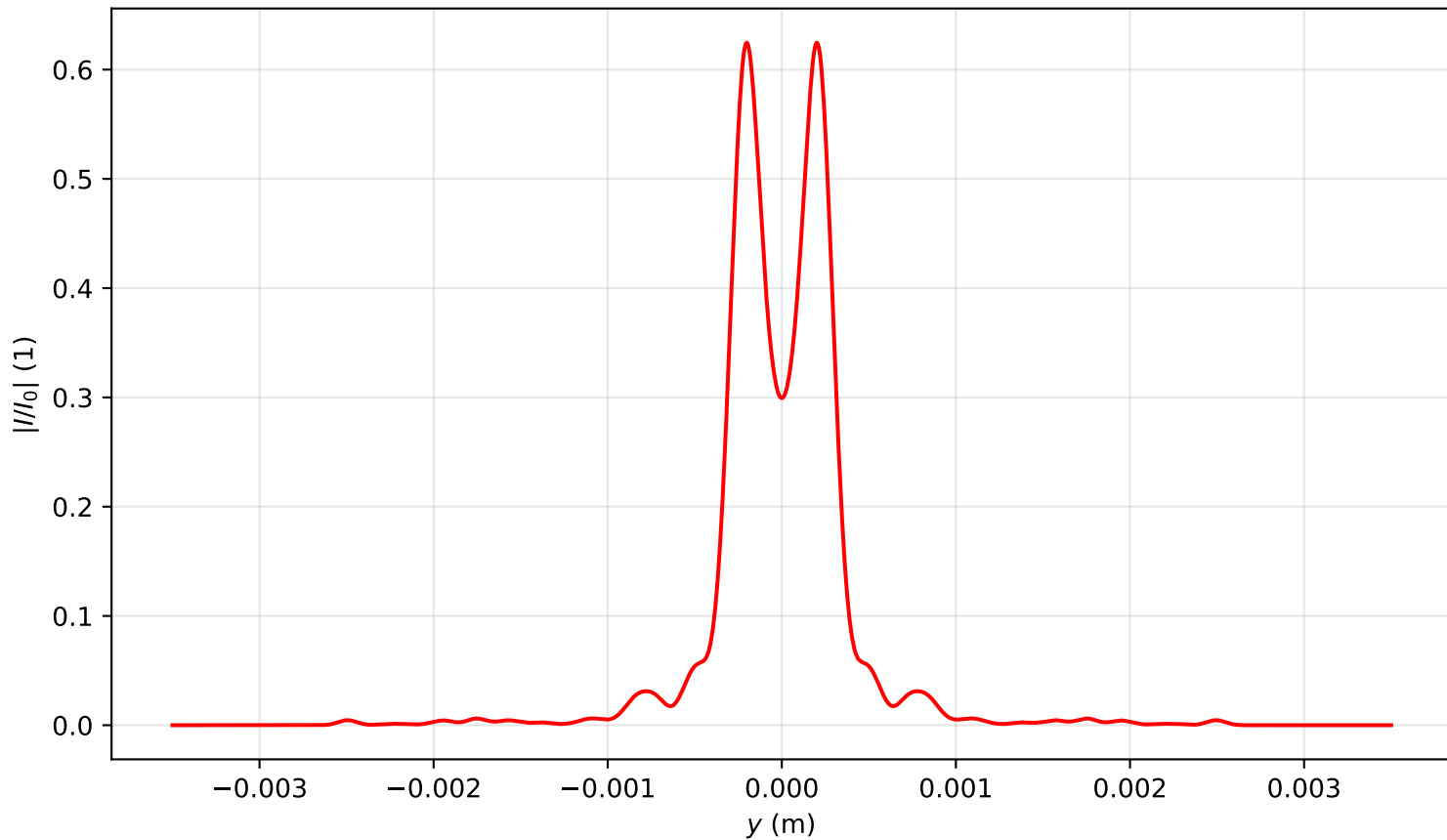
Intensity profile I(x=0, y, z=1.433)/I_0 , \text{Pin}=4.0\text{Pcr} , artificial time
